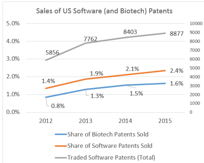
Figure 2: The Sale of US Software (and Biotechnology) Patents (2012–2015) 155
